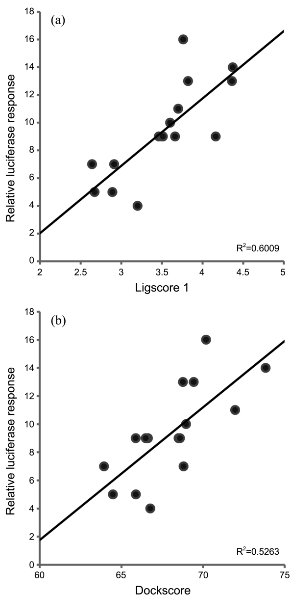
Figure 4. Correlation plots of (a) LigScore1 and (b) Dockscore of 16 carborane ligands with their relative luciferase response of ER \alpha in vitro .
