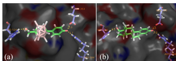
Figure 3. (a) The ER \alpha active site with the best docked pose of ligand 4c and (b) The ER \alpha active site with the crystal ligand E2 .
