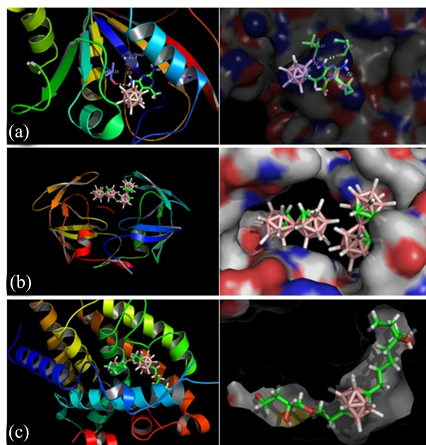
Figure 1. (a) The best docked pose of 2,4-diamino-5-(1- o -carboranylmethyl)-6-methylpyrimidine with DHFR, (b) The docked pose of cobalt bis(1,2-dicarbollide) with HIV protease, (c) The best docked pose of ( R )-stereoisomer of the ligand 3 with VDR.
