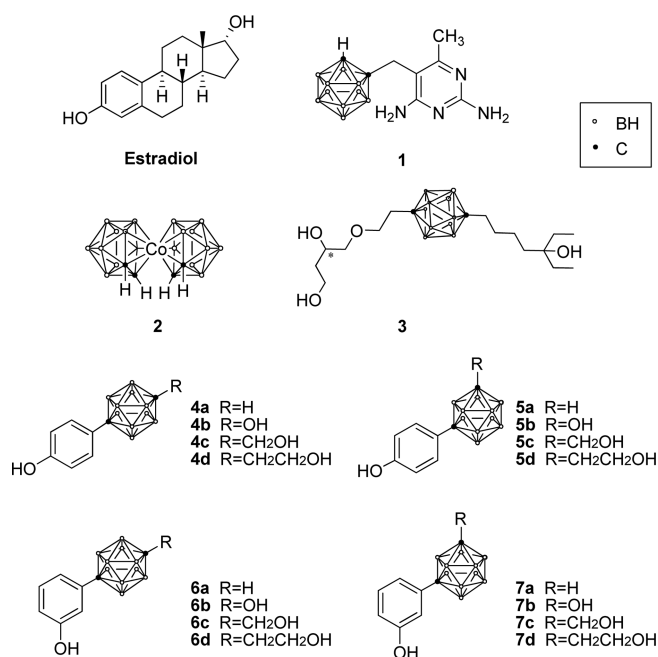
Figure 2. Chemical structures of carborane ligands for this study.
