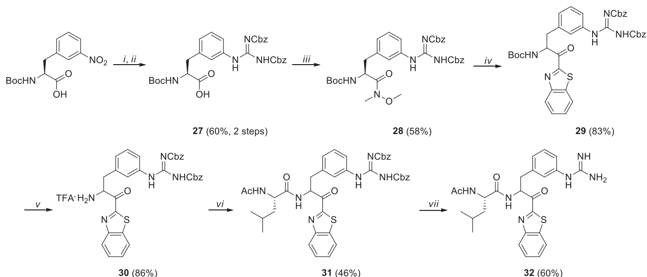
Scheme 5. Synthesis of m -phenylguanidine-based compound 32 a . a Reagents and conditions: (i) H 2 (gas), 10% Pd/C, MeOH, rt, 3 h; (ii) N,N' -bis(carbobenzoxy)-1H-pyrazole-1-carboxamide, Et 3 N, CH 2 Cl 2 , rt, 6 h; (iii) N,O -dimethylhydroxylamine HCl, HOBT, EDCI·HCl, DIPEA, THF, rt, 13 h; (iv) benzothiazole, TMEDA, n -BuLi, THF, −78 °C, 1.5 h; (v) TFA, triethylsilane, water, CH 2 Cl 2 , rt, 2 h; (vi) N -acetyl-L-leucine, HATU, DIPEA, rt, CH 2 Cl 2 , 5 h; (vii) TFA, thioanisole, rt, 12 h.
