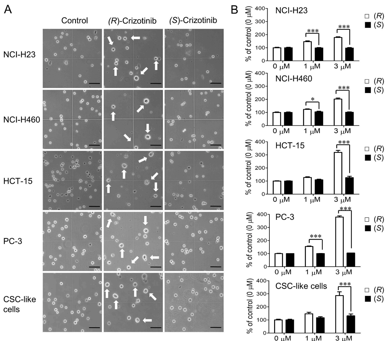
Fig. 3. (R)-crizotinib increases sizes of cancer and CSC-like cells. (A) NCI-H23, NCI-H460, HCT-15, PC-3, and PC-3 derived CSC-like cells were incubated with or without 3 \mu M of (R)- or (S)-crizotinib for 72 h. They were then trypsinized, suspended in PBS (pH 7.4), and observed under an inverted microscope. White arrows indicate cells increased in sizes. Scale bar: 100 \mu m. (B) Sizes of cells incubated with (R)- or (S)-crizotinib at various concentrations (0, 1, and 3 \mu M) for 72 h were measured (n = 3) using Image J2 program. Data are presented as mean \pm SD. **, p < 0.01 ; ***, p < 0.001 .
